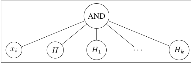
Figure 2: merging of the ANDs
