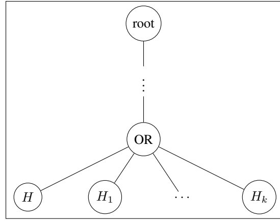
Figure 1: x_i is in one of the H_j
